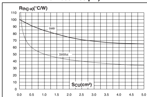
Figure 17. Thermal resistance junction to ambient versus copper surface under each lead, SMB, SMBflat (epoxy printed board FR4, copper thickness = 35 \mu m)
