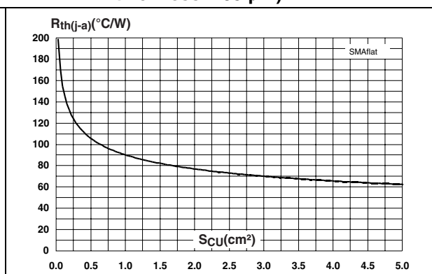
Figure 18. Thermal resistance junction to ambient versus copper surface under each lead, SMAflat (epoxy printed board FR4, copper thickness = 35 \mu m)
