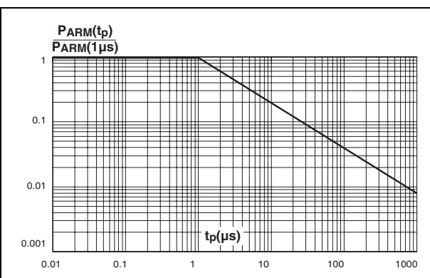
Figure 8. Normalized avalanche power derating versus pulse duration
